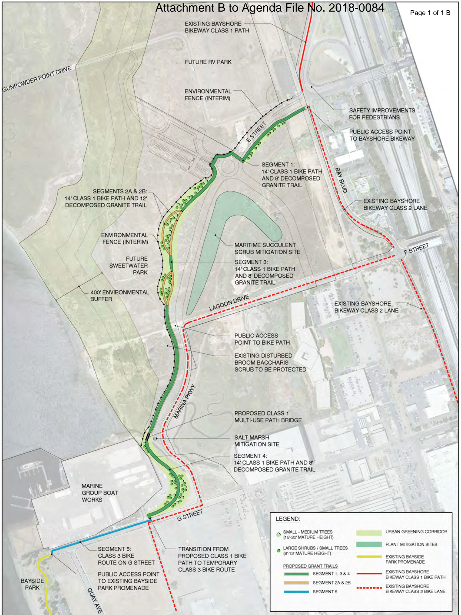
SITE PLAN SWEETWATER BICYCLE PATH AND PEDESTRIAN PROMENADE - URBAN GREENING STRATEGY
