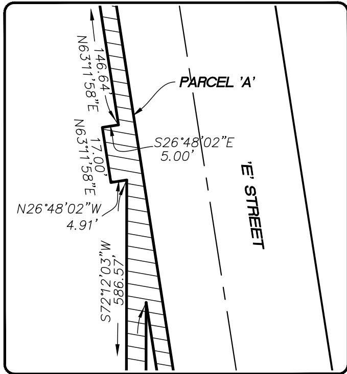
DETAIL 'A' SCALE: 1"=30'
